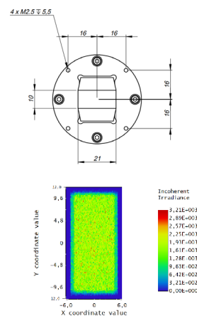
outline and homogeneity of module 3600W 21x10
